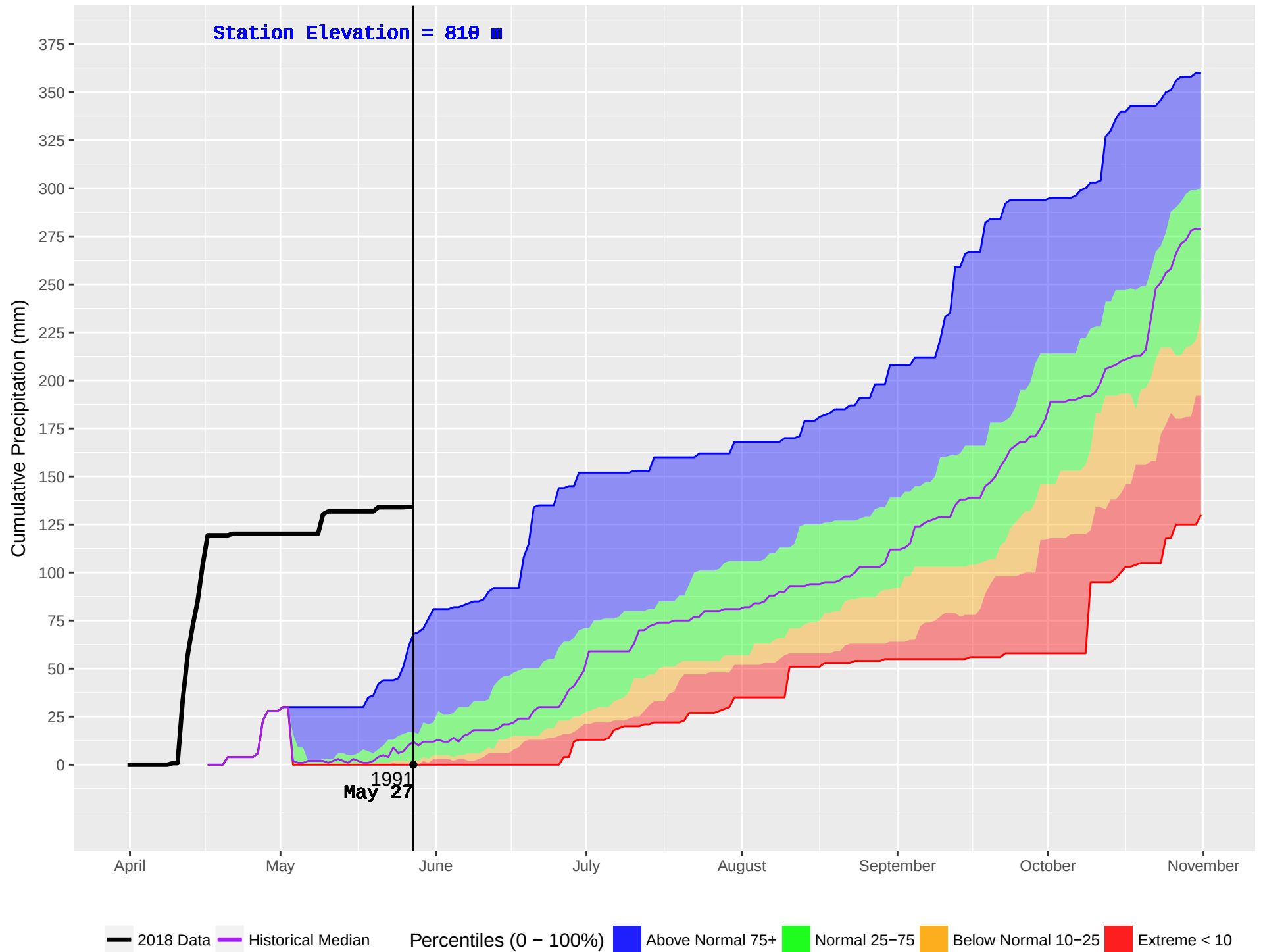
MCBRIDE LAKE (180) : Historical (1990–2016) and Current (2018) Noon Cumulative Precipitation
