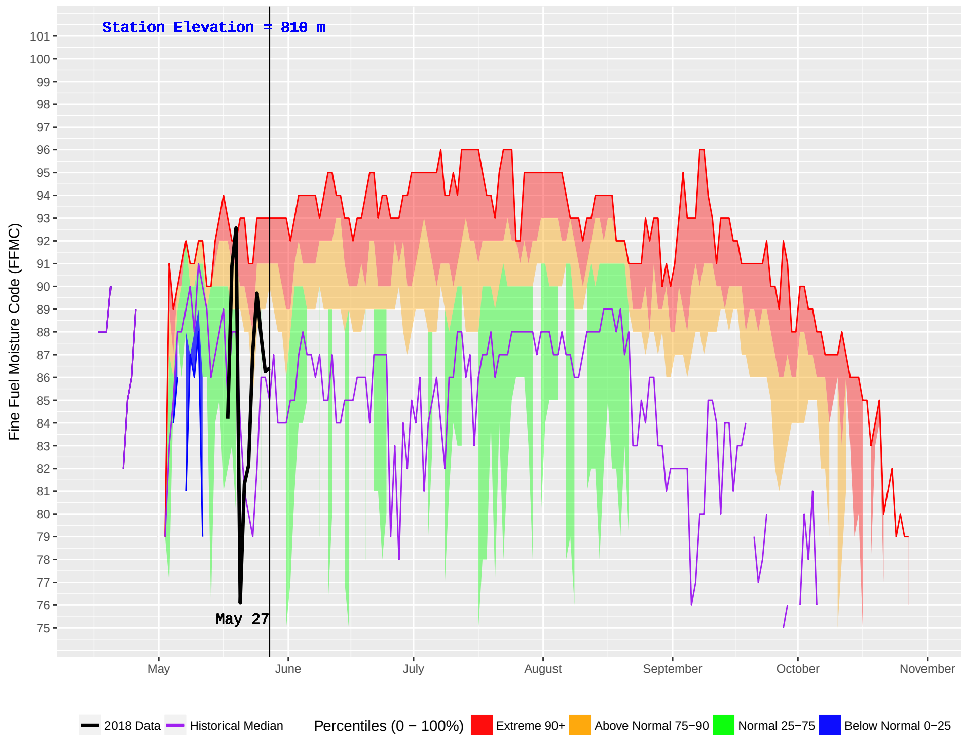
MCBRIDE LAKE (180) : Historical (1990–2016) and Current (2018) Noon Fine Fuel Moisture Code (FFMC)
