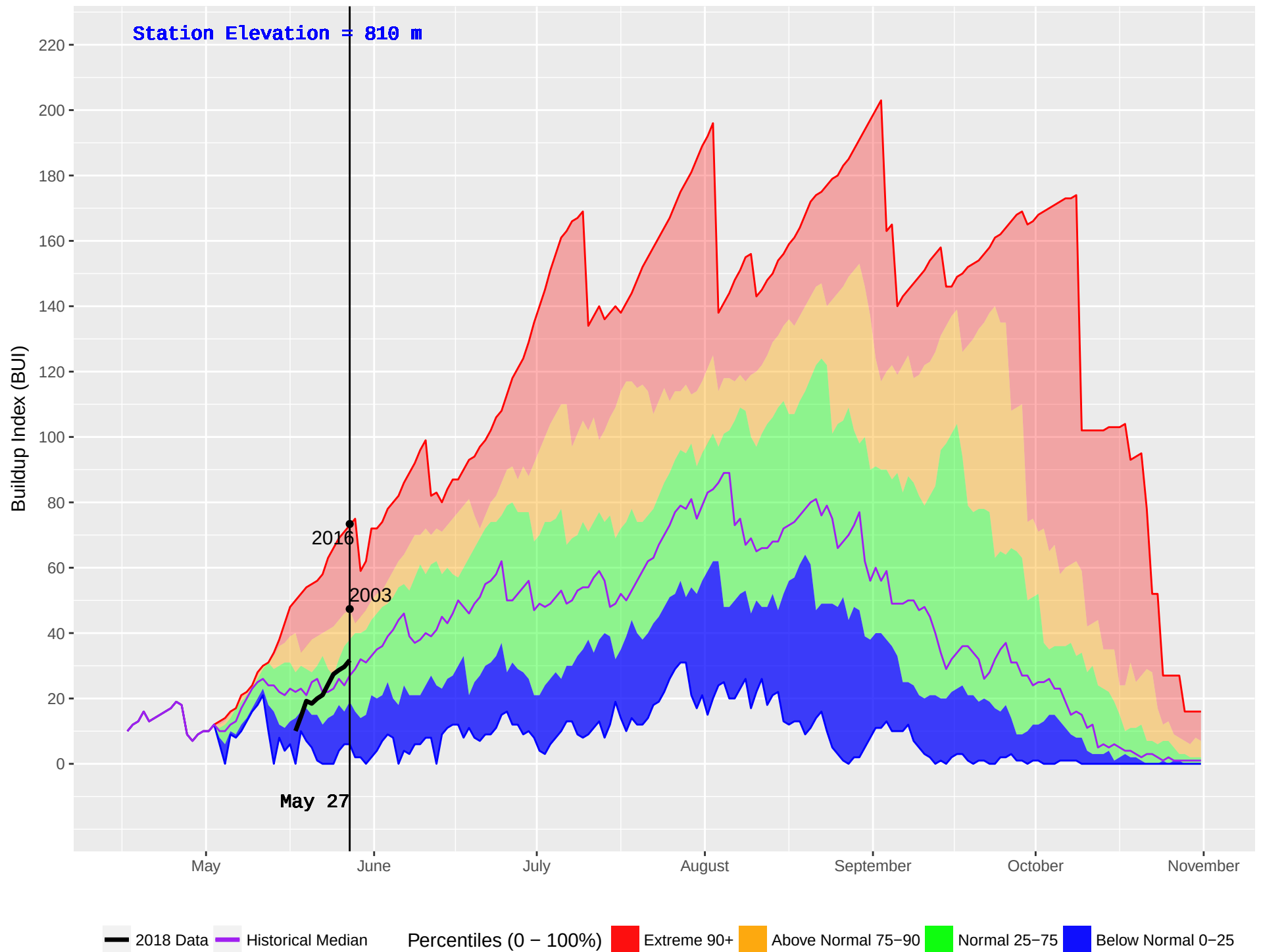
MCBRIDE LAKE (180) : Historical (1990–2016) and Current (2018) Noon Buildup Index (BUI)
