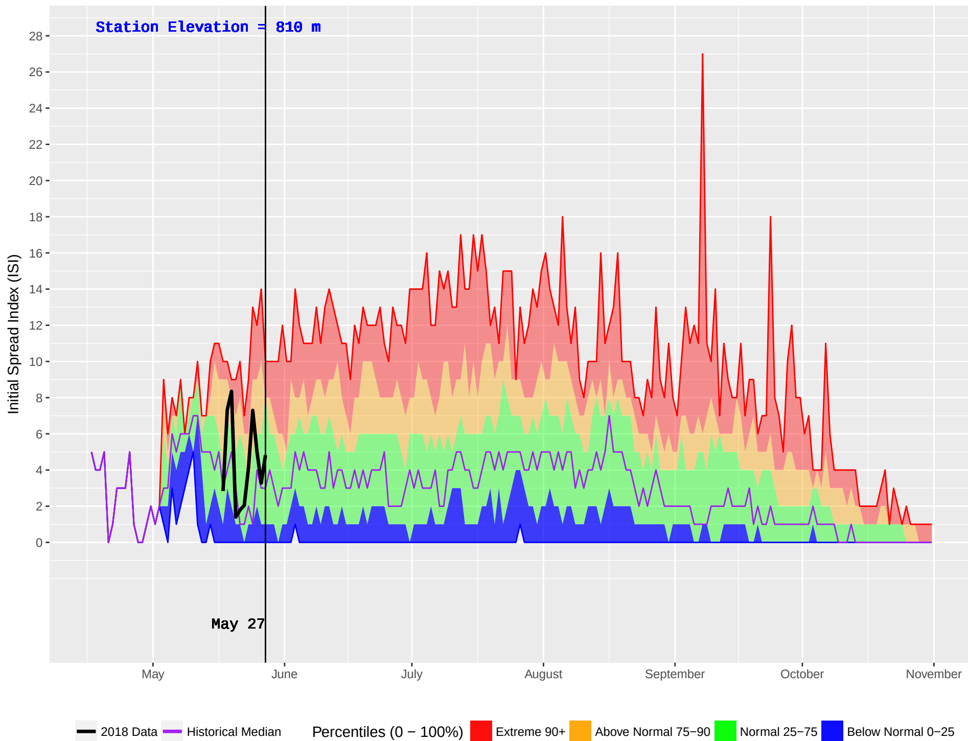
MCBRIDE LAKE (180) : Historical (1990–2016) and Current (2018) Noon Initial Spread Index (ISI)
