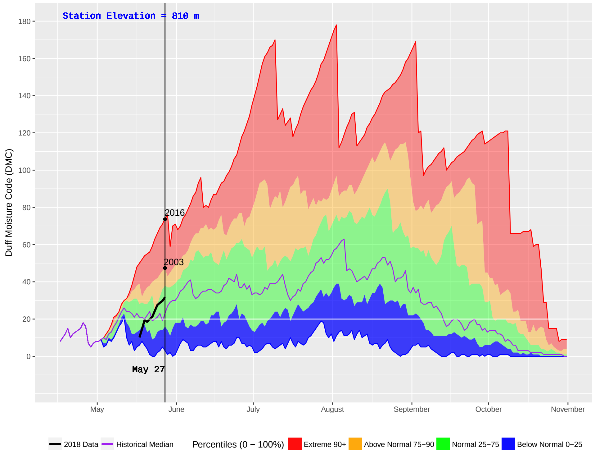
MCBRIDE LAKE (180) : Historical (1990–2016) and Current (2018) Noon Duff Moisture Code (DMC)
